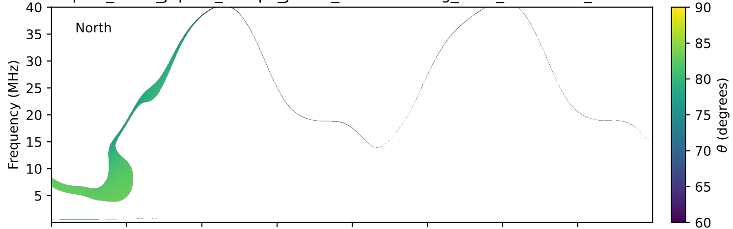
expres_earth_jupiter_europa_jrm33_lossc-wid1deg_3kev_20241216_v11.cdf
