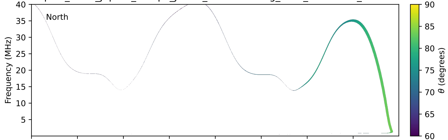
expres_earth_jupiter_europa_jrm33_lossc-wid1deg_3kev_20241206_v11.cdf
