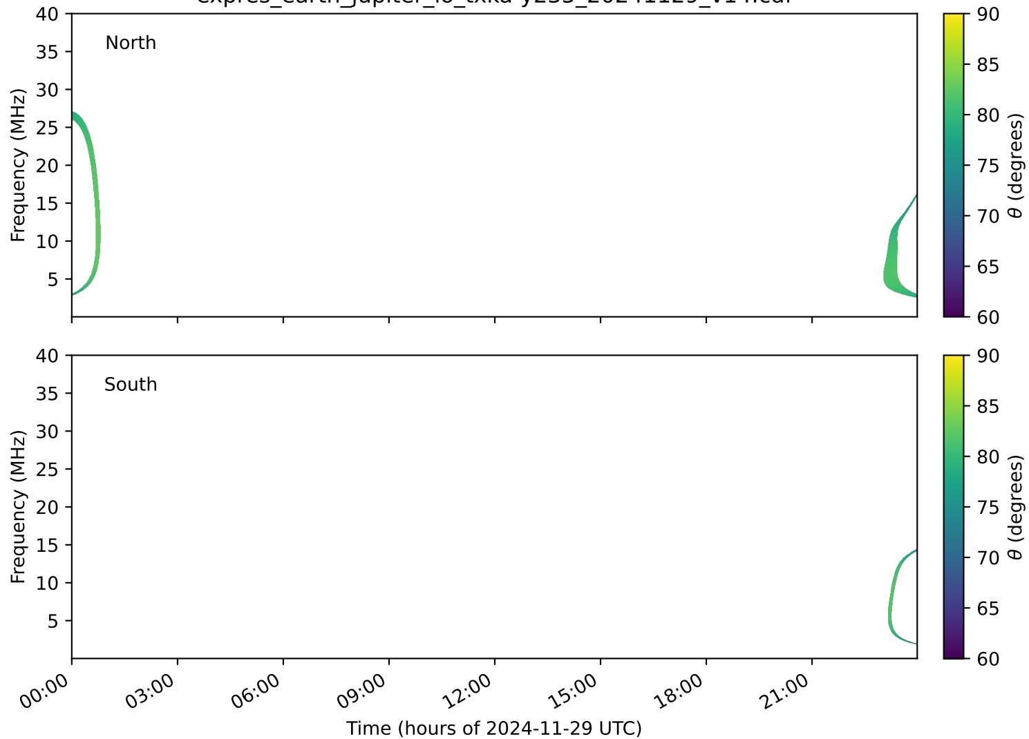
expres_earth_jupiter_io_txka-y235_20241129_v14.cdf
