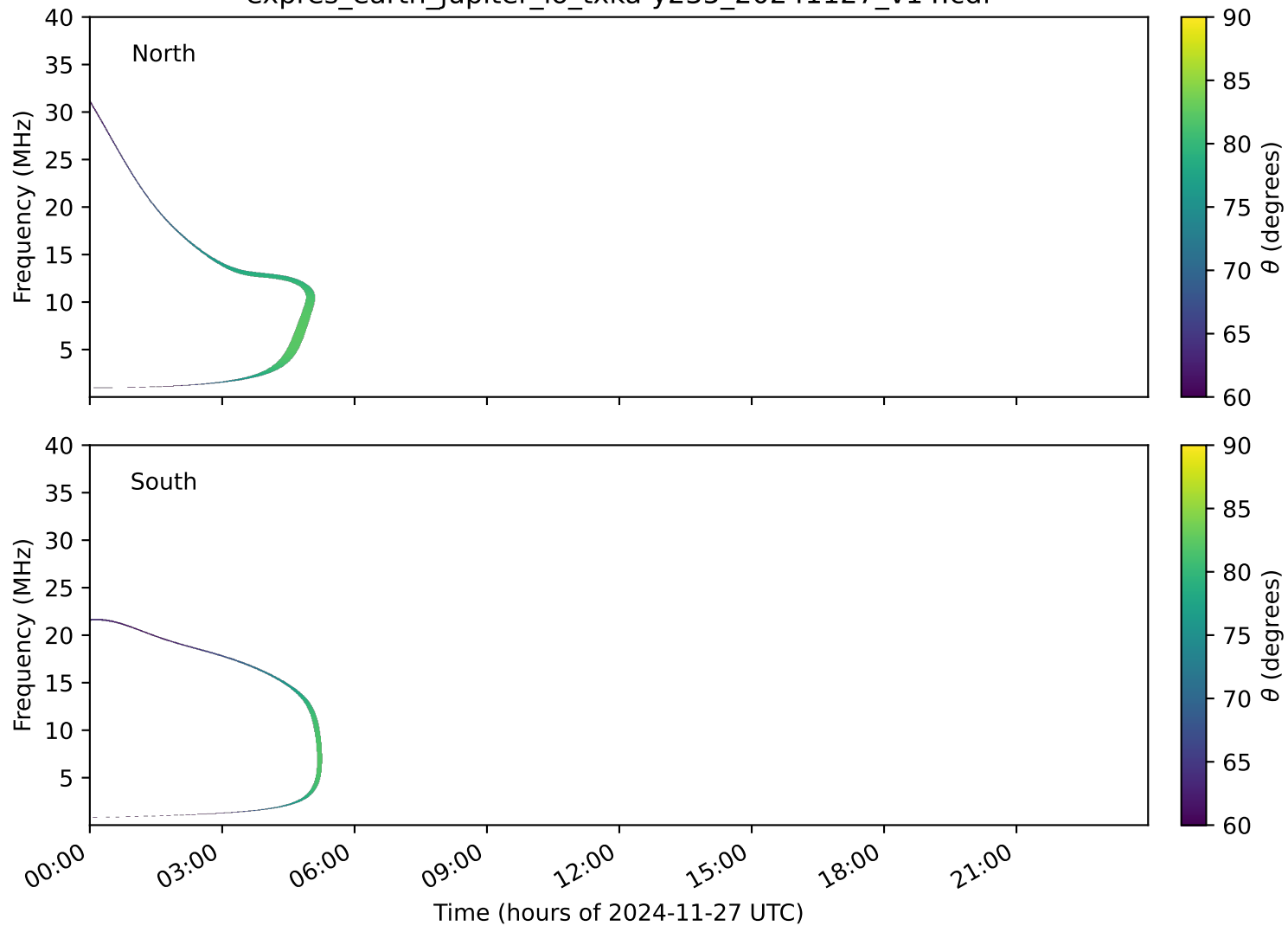
expres_earth_jupiter_io_txka-y235_20241127_v14.cdf
