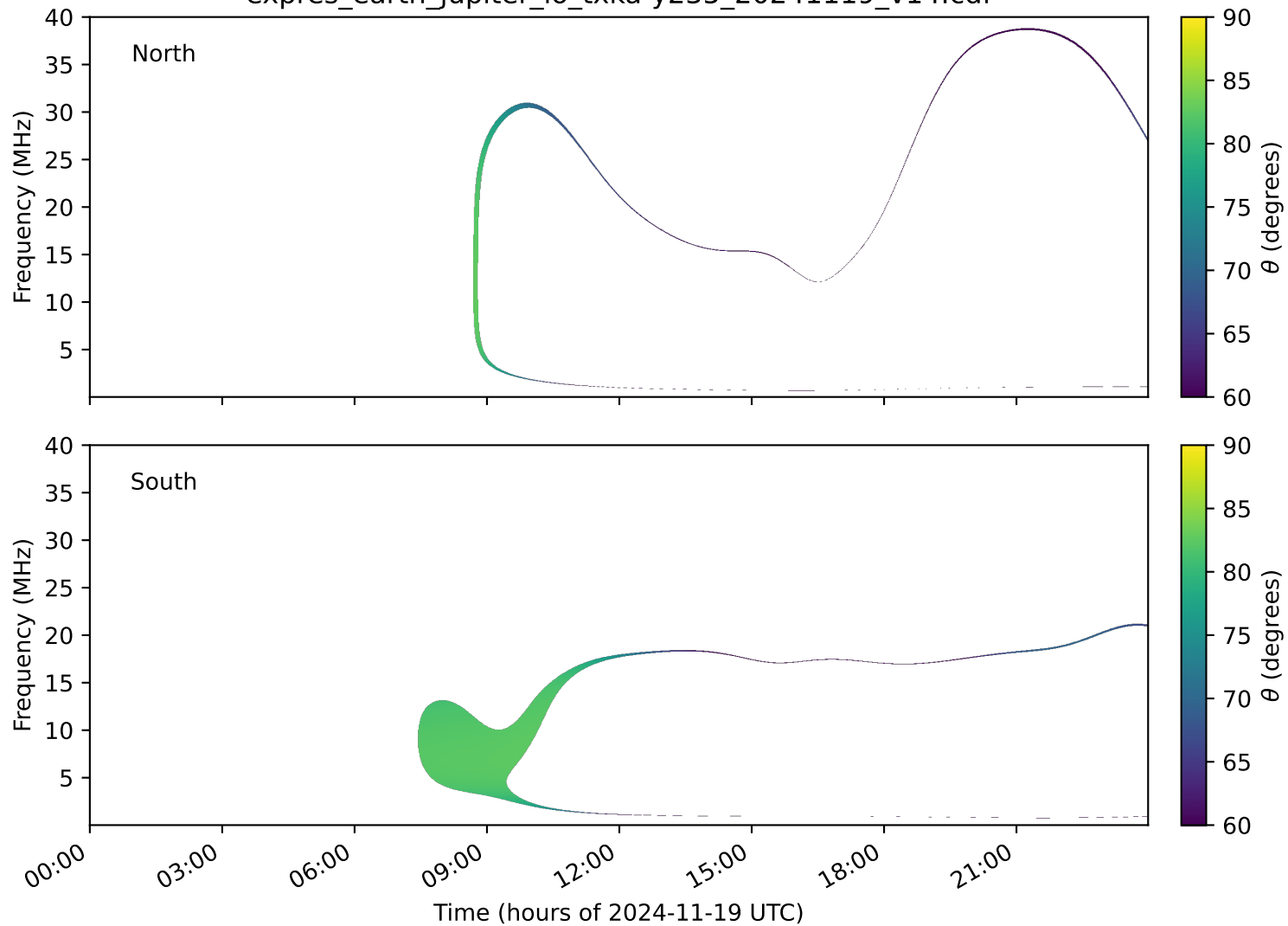
expres_earth_jupiter_io_txka-y235_20241119_v14.cdf
