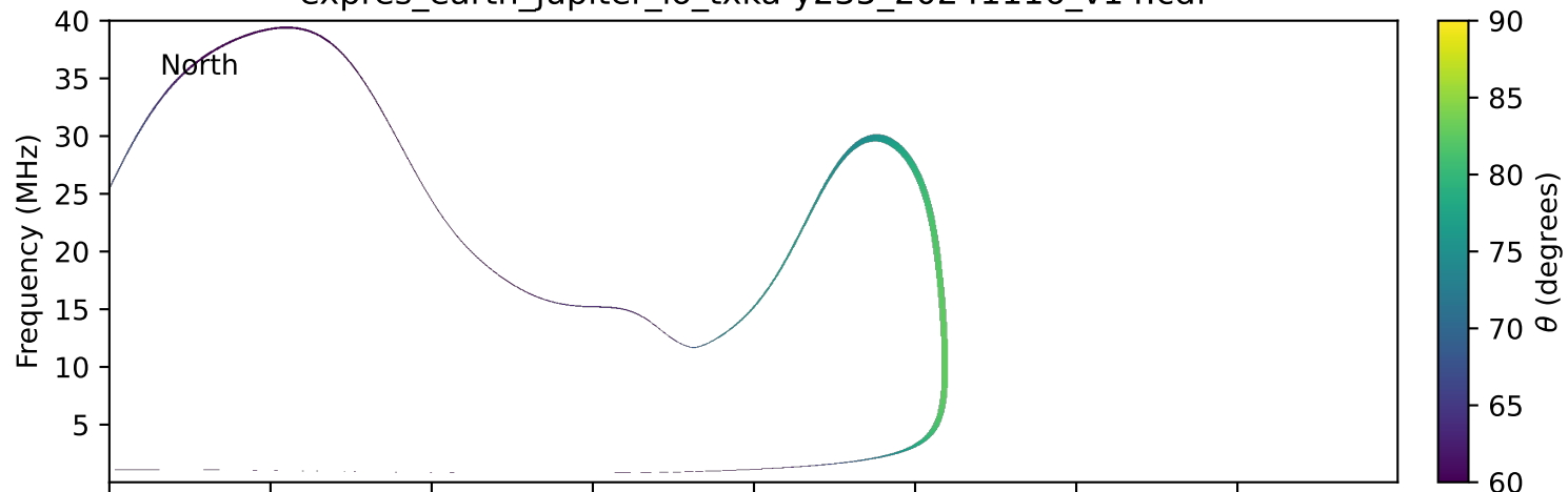
expres_earth_jupiter_io_txka-y235_20241116_v14.cdf
