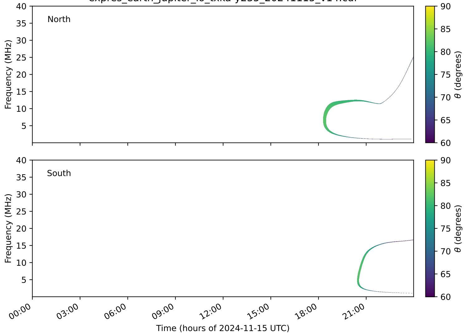
expres_earth_jupiter_io_txka-y235_20241115_v14.cdf
