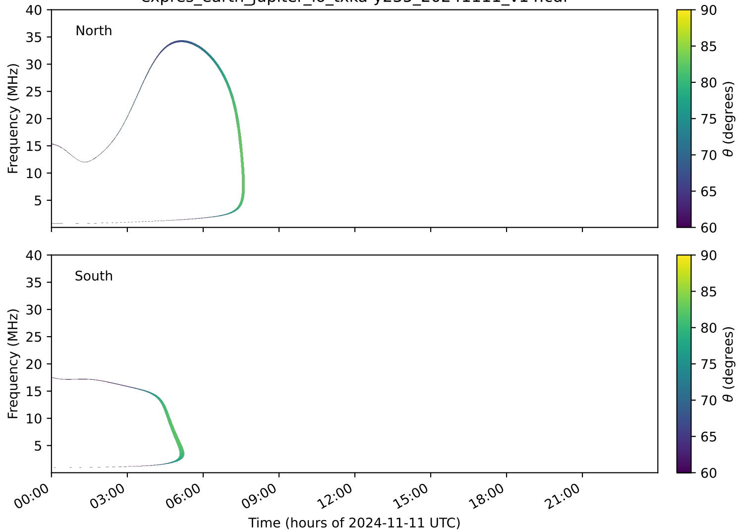
expres_earth_jupiter_io_txka-y235_20241111_v14.cdf
