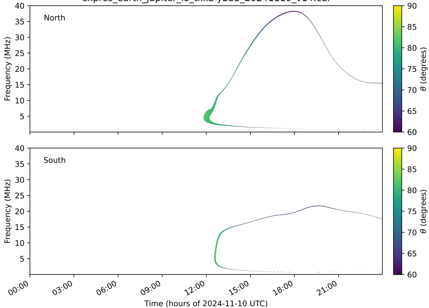
expres_earth_jupiter_io_txka-y235_20241110_v14.cdf
