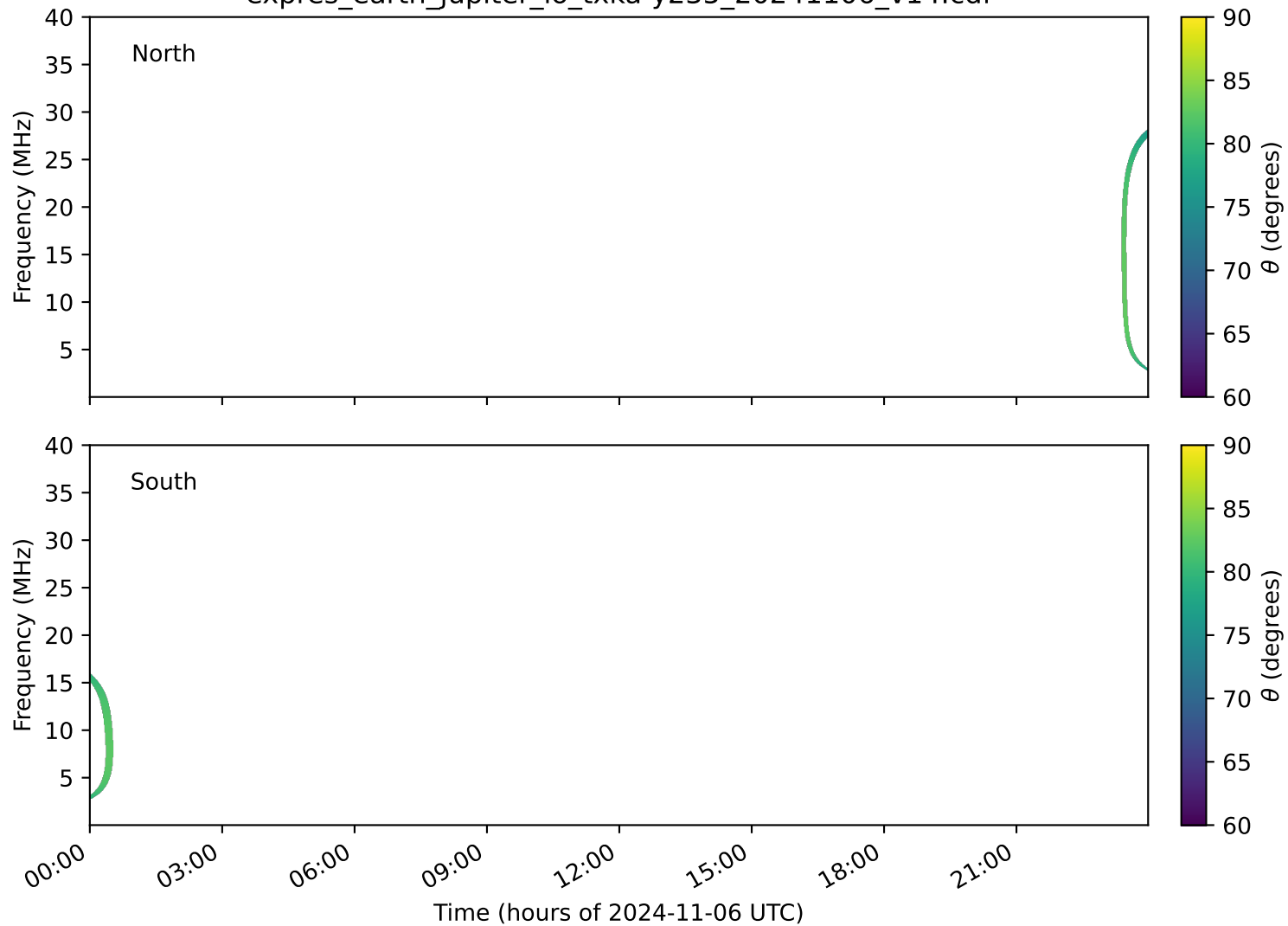
expres_earth_jupiter_io_txka-y235_20241106_v14.cdf
