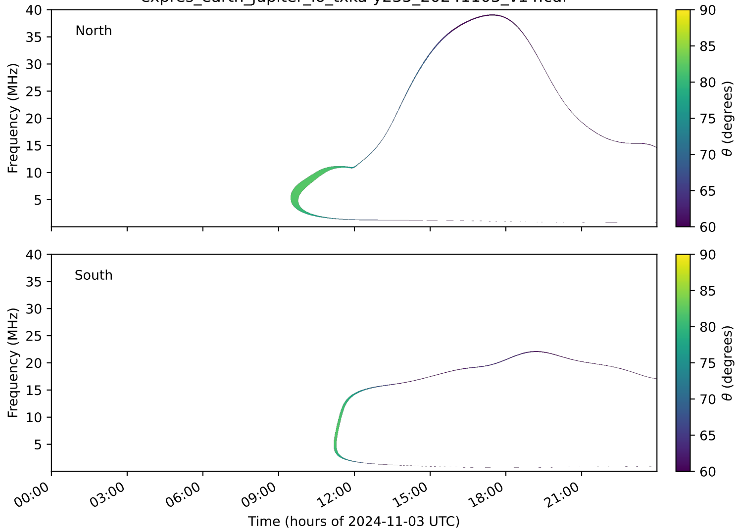
expres_earth_jupiter_io_txka-y235_20241103_v14.cdf
