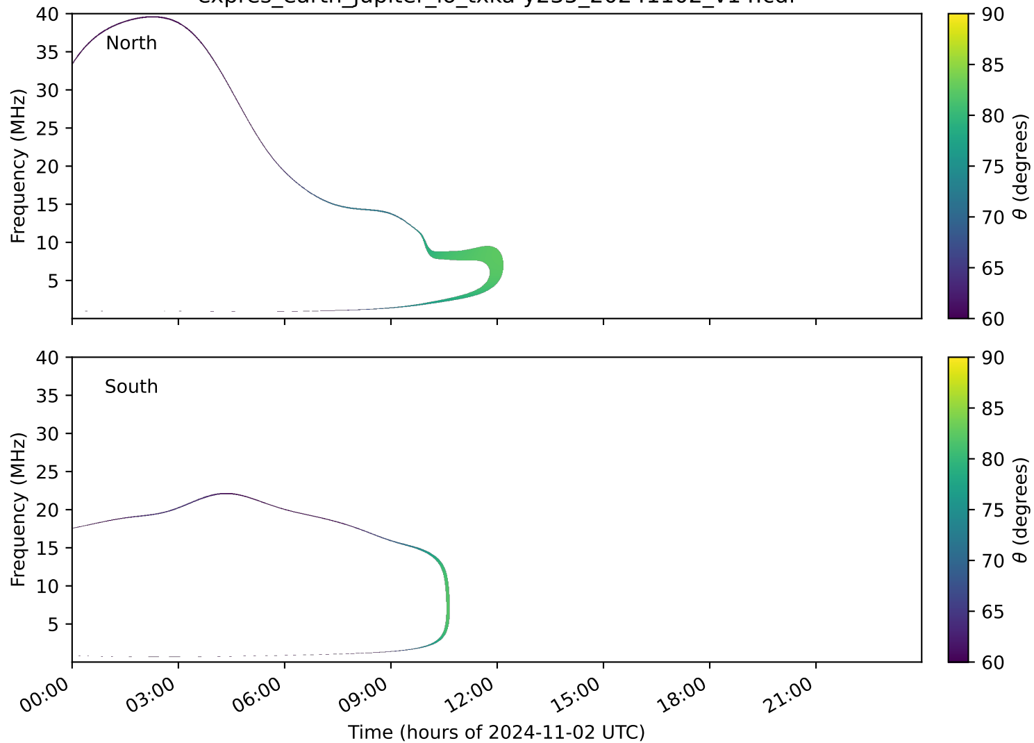
expres_earth_jupiter_io_txka-y235_20241102_v14.cdf
