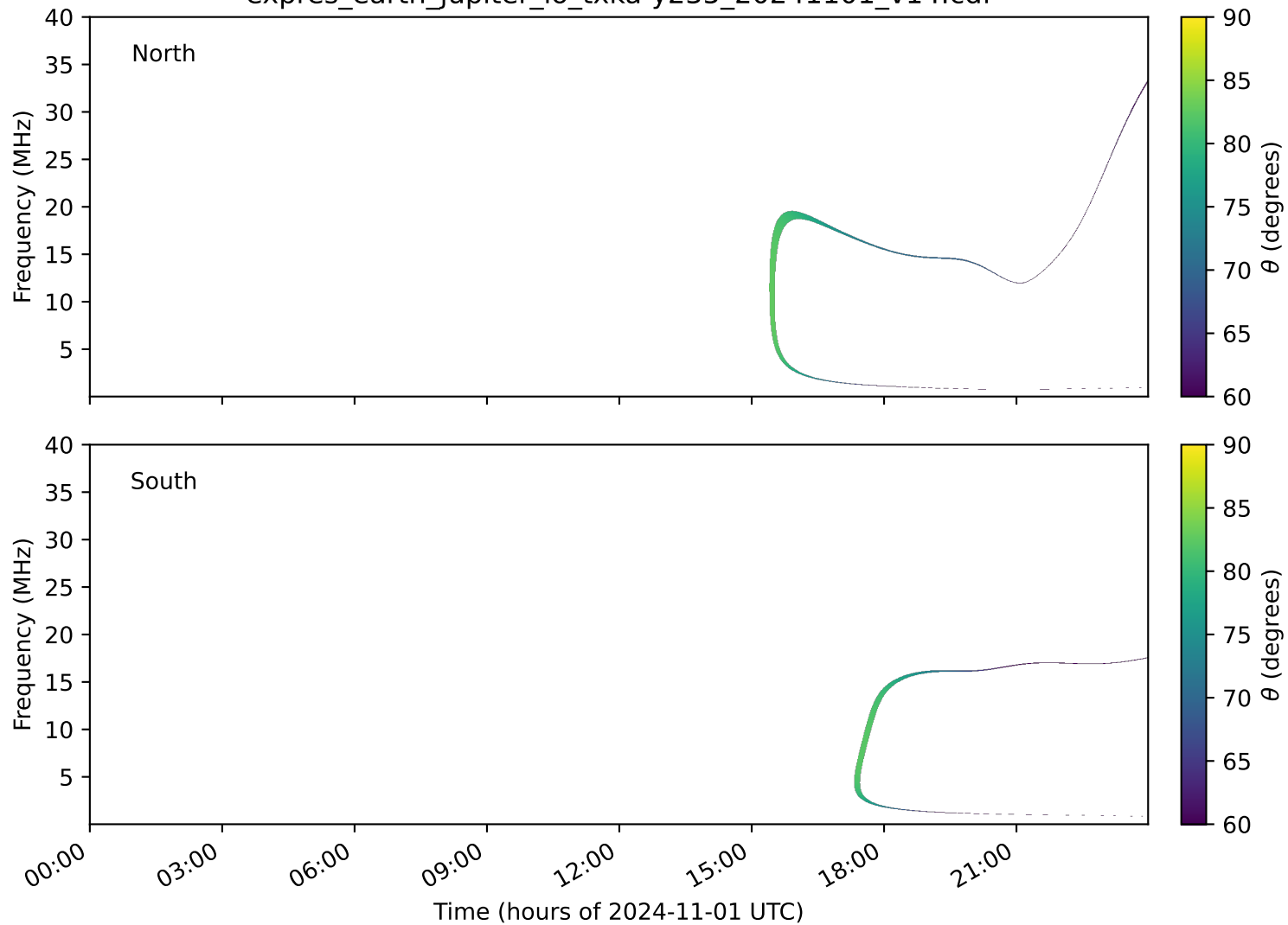
expres_earth_jupiter_io_txka-y235_20241101_v14.cdf
