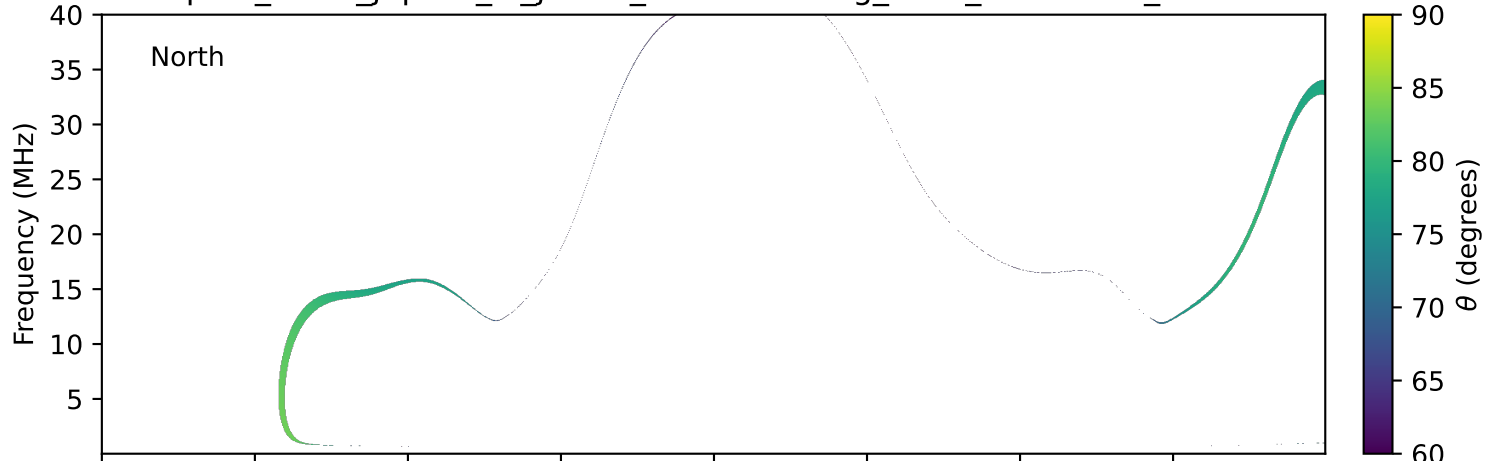
expres_earth_jupiter_io_jrm33_lossc-wid1deg_3kev_20241128_v11.cdf
