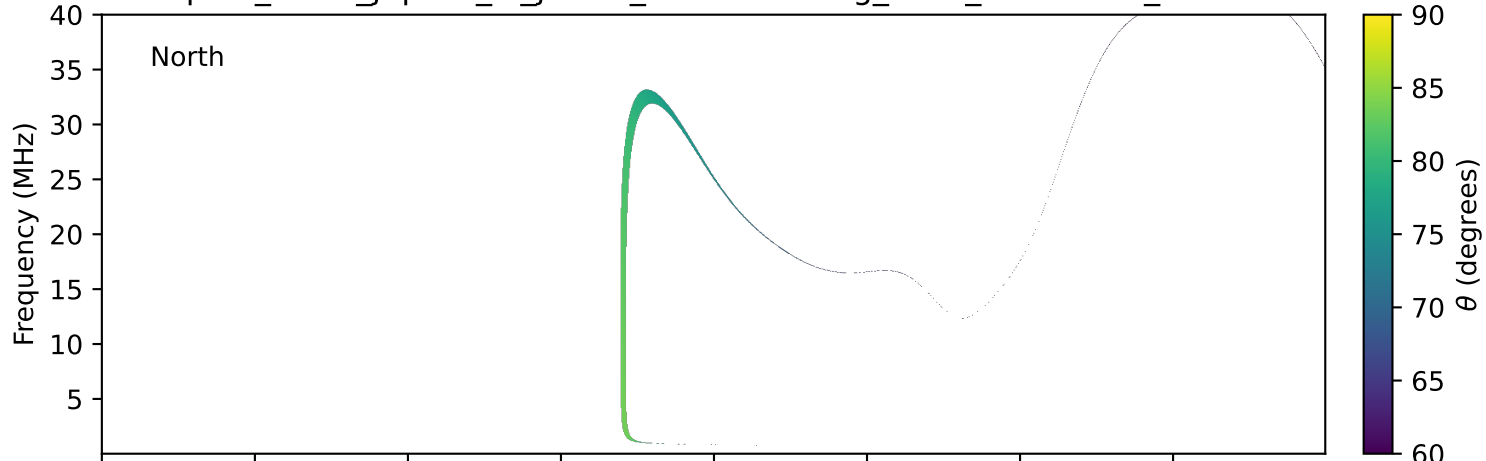
expres_earth_jupiter_io_jrm33_lossc-wid1deg_3kev_20241126_v11.cdf
