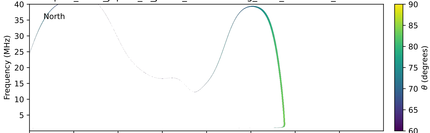
expres_earth_jupiter_io_jrm33_lossc-wid1deg_3kev_20241123_v11.cdf
