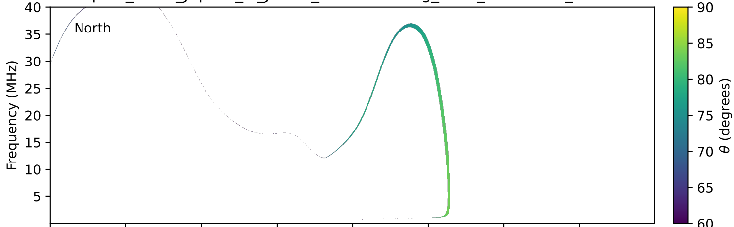
expres_earth_jupiter_io_jrm33_lossc-wid1deg_3kev_20241116_v11.cdf
