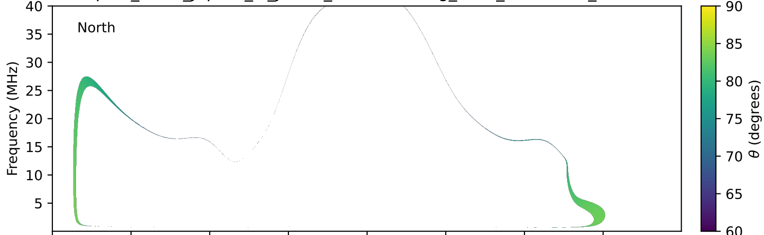
expres_earth_jupiter_io_jrm33_lossc-wid1deg_3kev_20241114_v11.cdf
