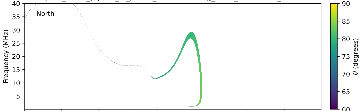
expres_earth_jupiter_io_jrm33_lossc-wid1deg_3kev_20241109_v11.cdf
