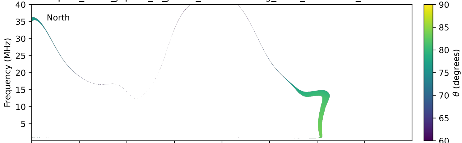
expres_earth_jupiter_io_jrm33_lossc-wid1deg_3kev_20241107_v11.cdf
