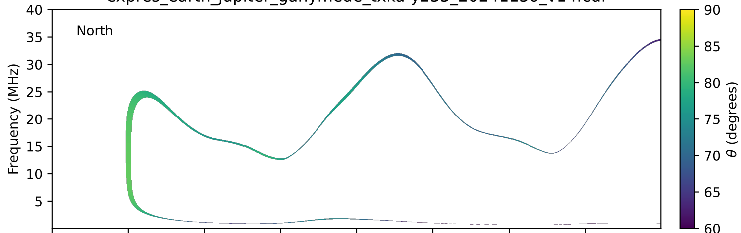
expres_earth_jupiter_ganymede_txka-y235_20241130_v14.cdf
