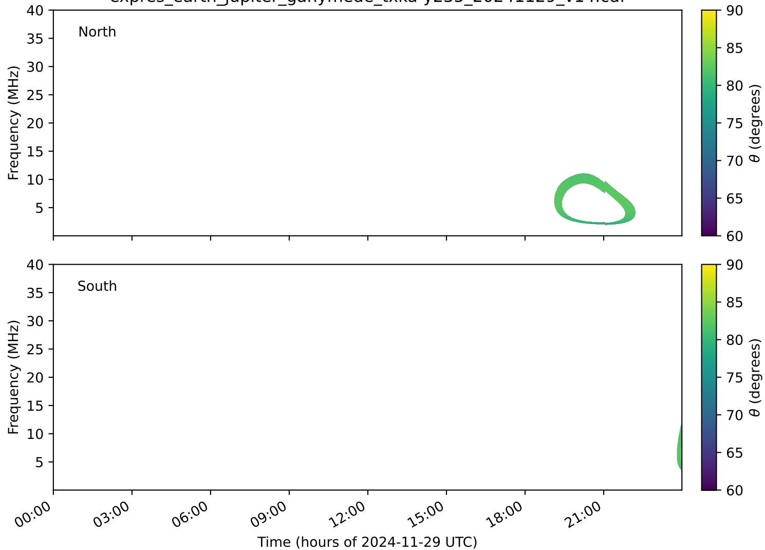
expres_earth_jupiter_ganymede_txka-y235_20241129_v14.cdf
