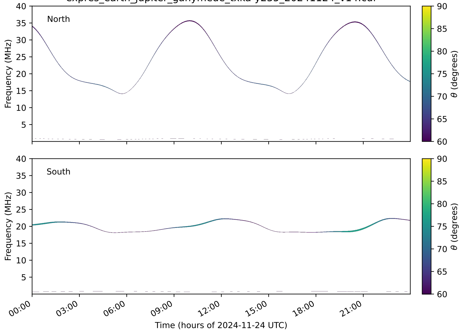
expres_earth_jupiter_ganymede_txka-y235_20241124_v14.cdf
