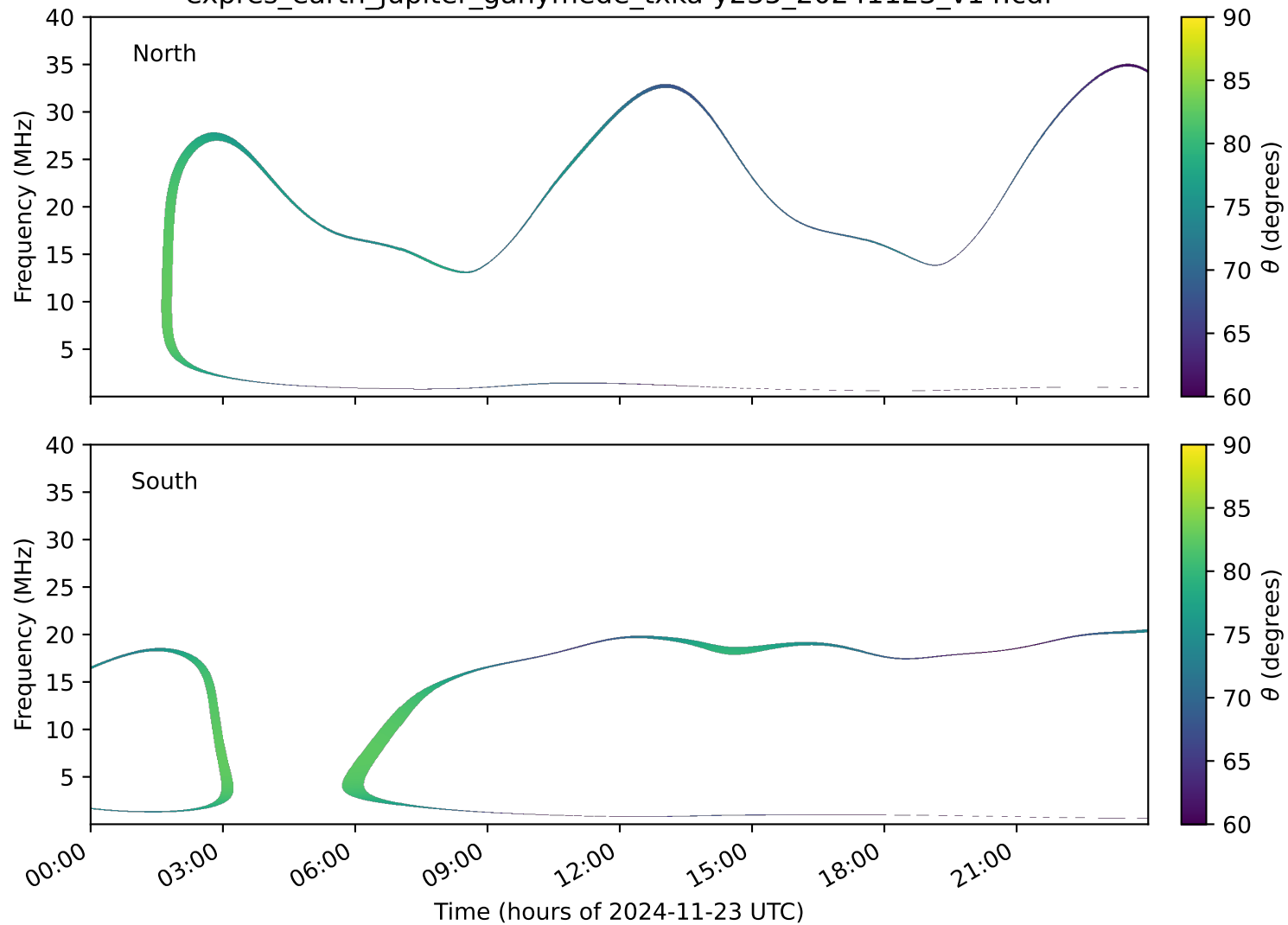
expres_earth_jupiter_ganymede_txka-y235_20241123_v14.cdf
