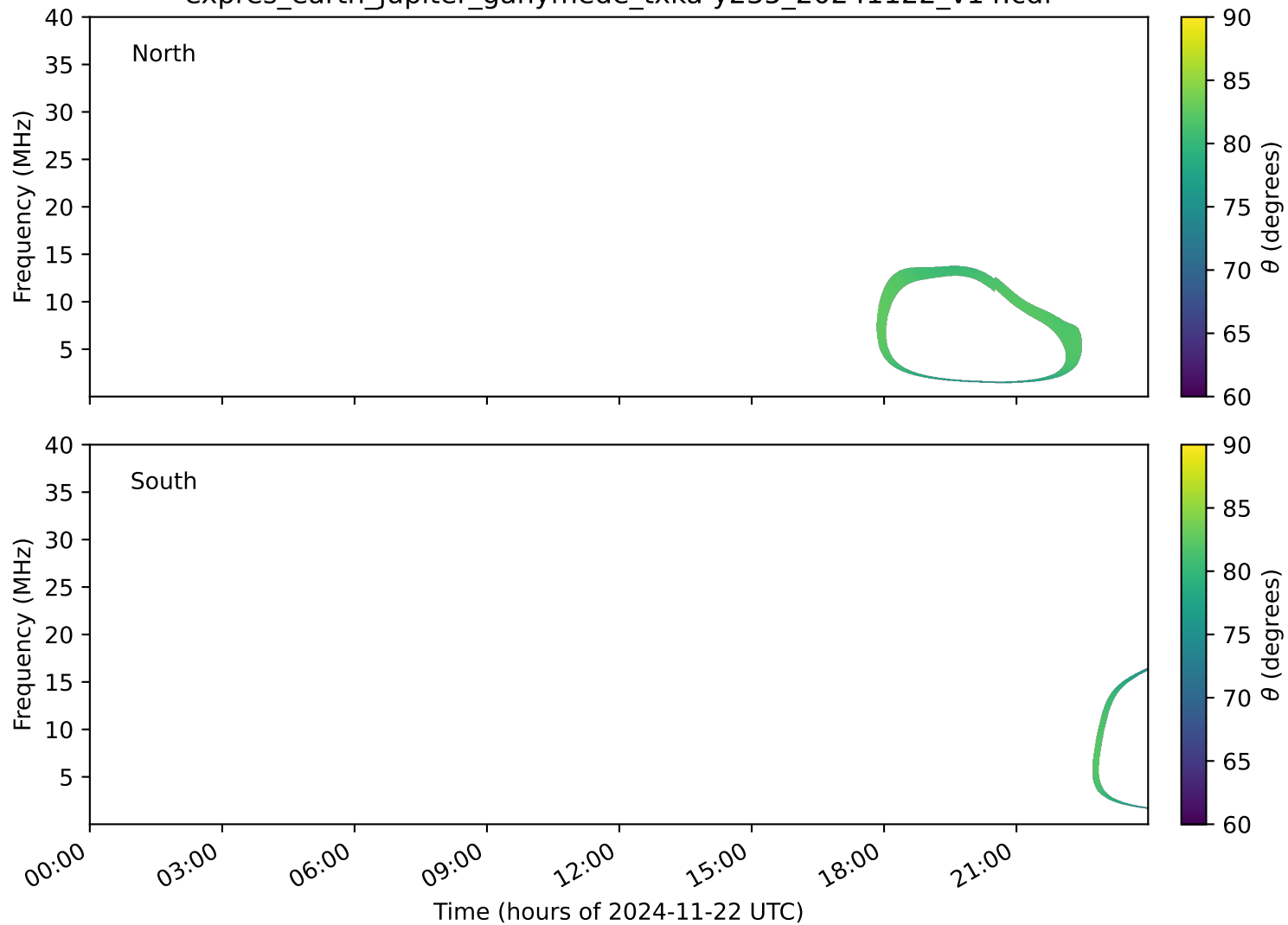
expres_earth_jupiter_ganymede_txka-y235_20241122_v14.cdf
