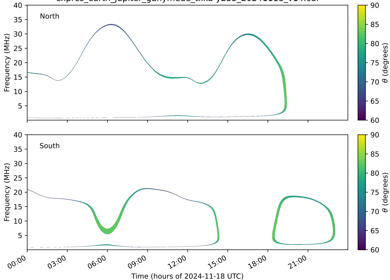
expres_earth_jupiter_ganymede_txka-y235_20241118_v14.cdf
