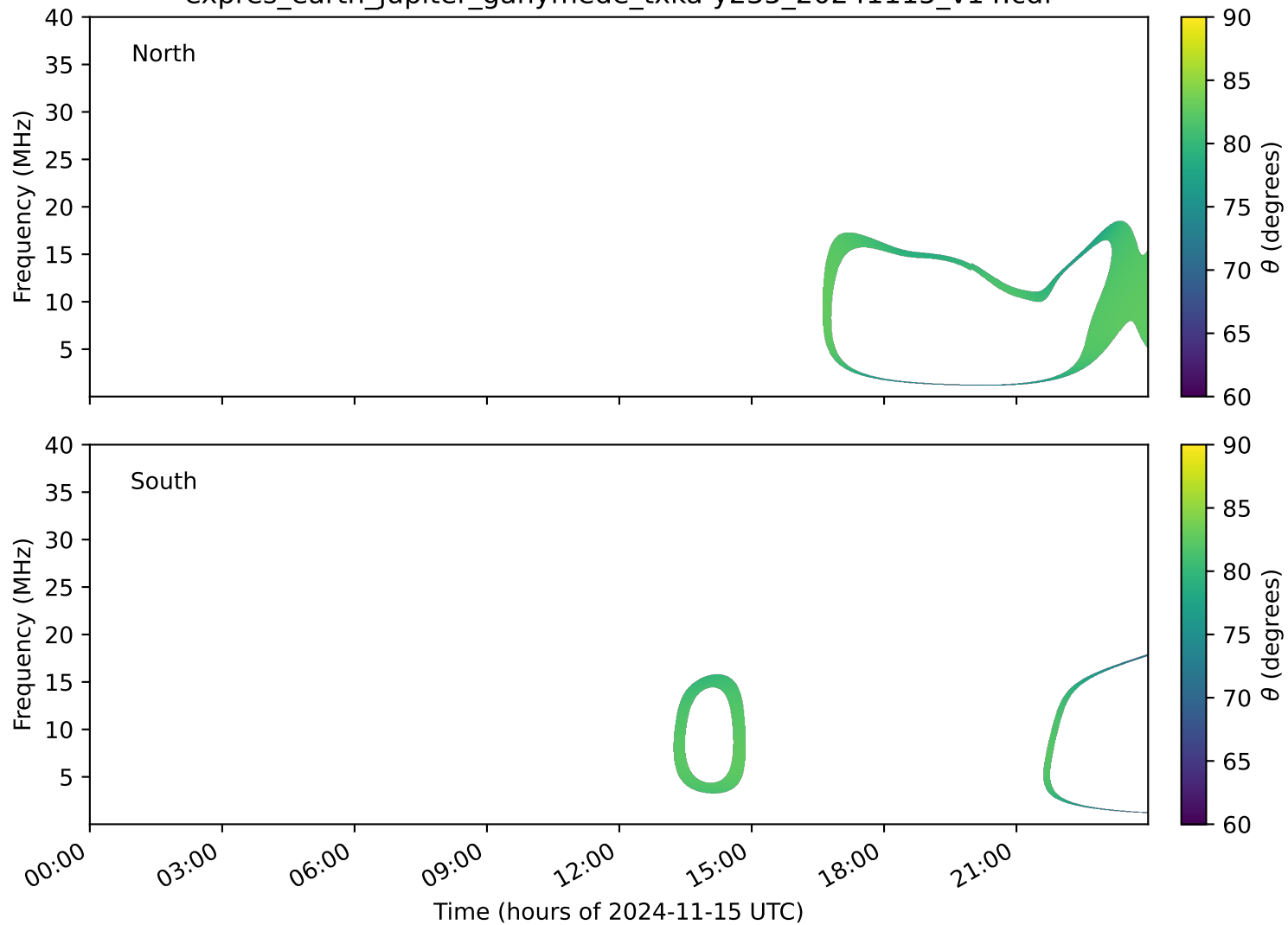
expres_earth_jupiter_ganymede_txka-y235_20241115_v14.cdf
