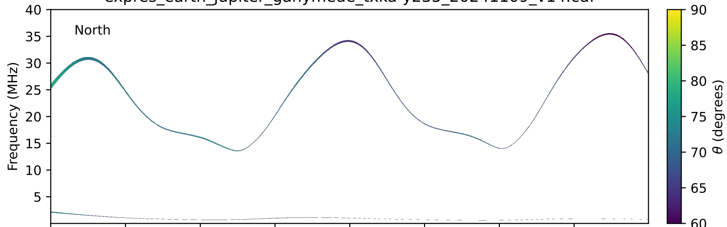
expres_earth_jupiter_ganymede_txka-y235_20241109_v14.cdf
