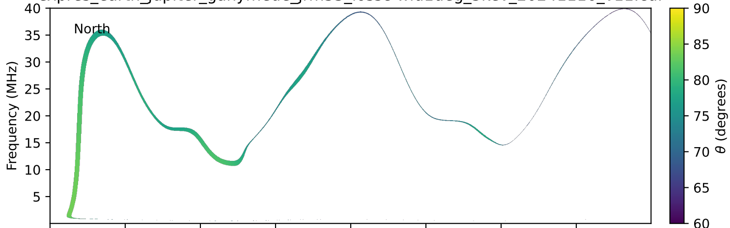
expres_earth_jupiter_ganymede_jrm33_lossc-wid1deg_3kev_20241116_v11.cdf
