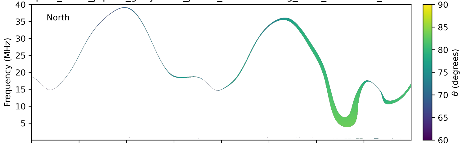
expres_earth_jupiter_ganymede_jrm33_lossc-wid1deg_3kev_20241111_v11.cdf
