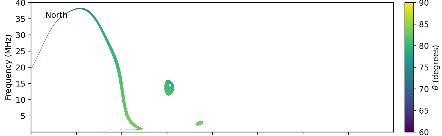
expres_earth_jupiter_europa_jrm33_lossc-wid1deg_3kev_20241126_v11.cdf
