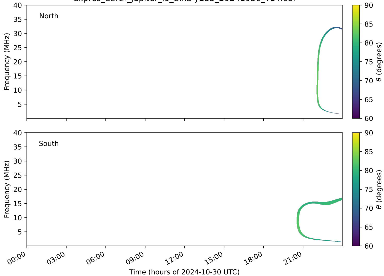
expres_earth_jupiter_io_txka-y235_20241030_v14.cdf
