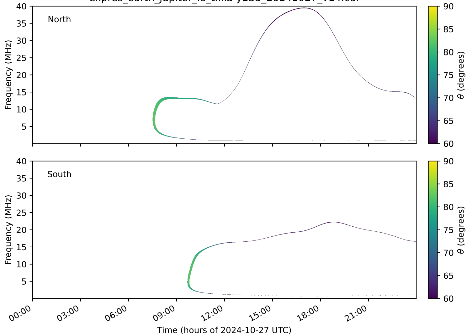
expres_earth_jupiter_io_txka-y235_20241027_v14.cdf
