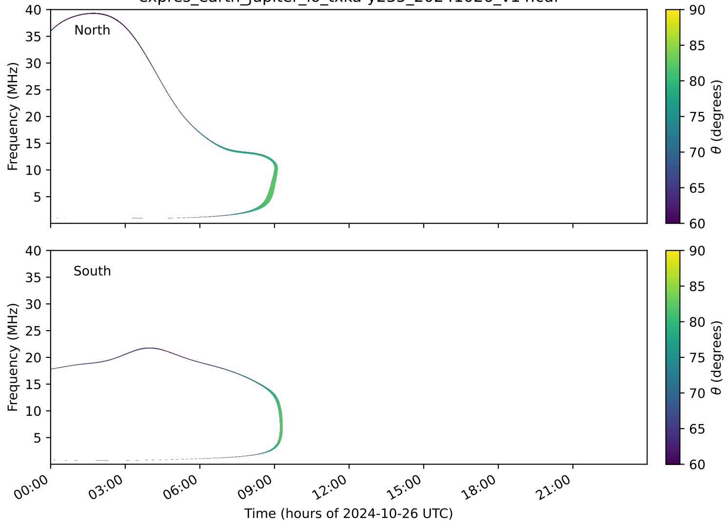
expres_earth_jupiter_io_txka-y235_20241026_v14.cdf
