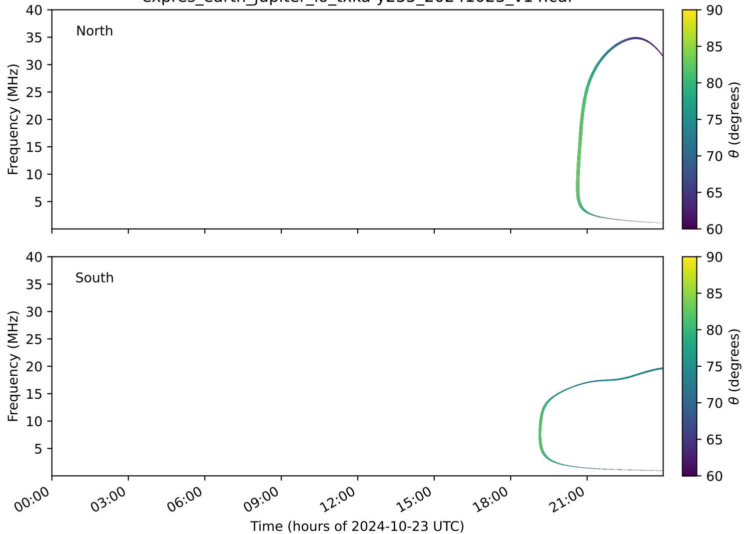
expres_earth_jupiter_io_txka-y235_20241023_v14.cdf
