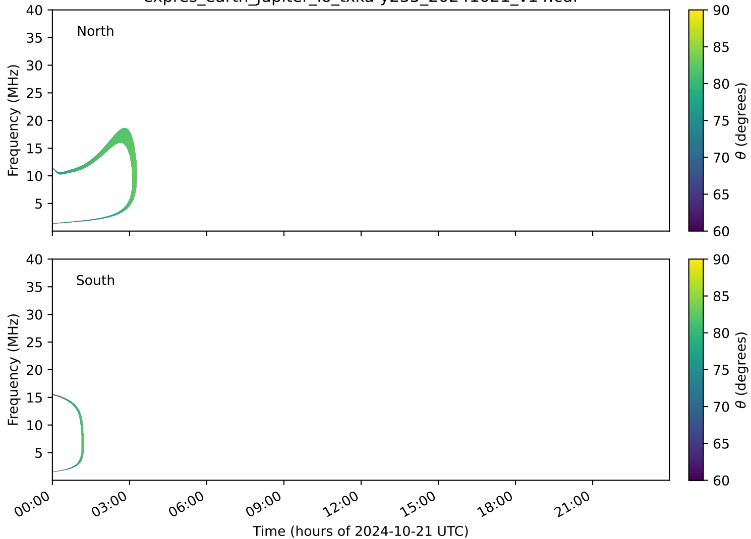
expres_earth_jupiter_io_txka-y235_20241021_v14.cdf
