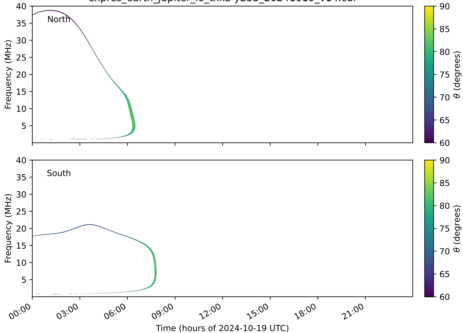
expres_earth_jupiter_io_txka-y235_20241019_v14.cdf
