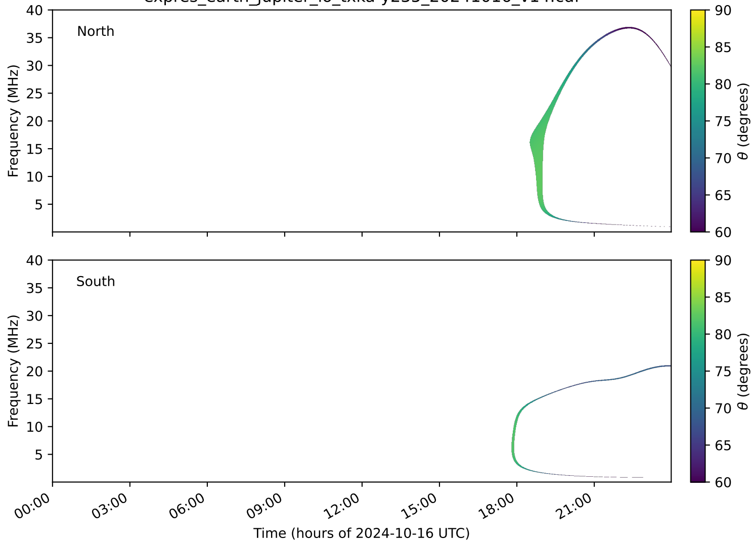
expres_earth_jupiter_io_txka-y235_20241016_v14.cdf
