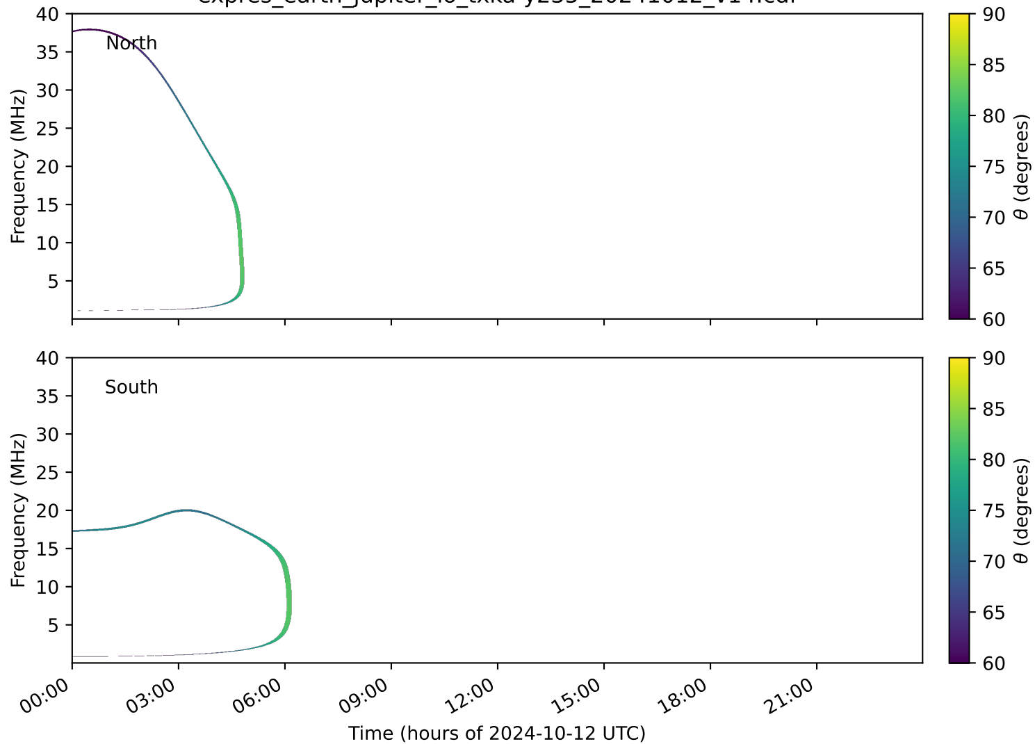
expres_earth_jupiter_io_txka-y235_20241012_v14.cdf
