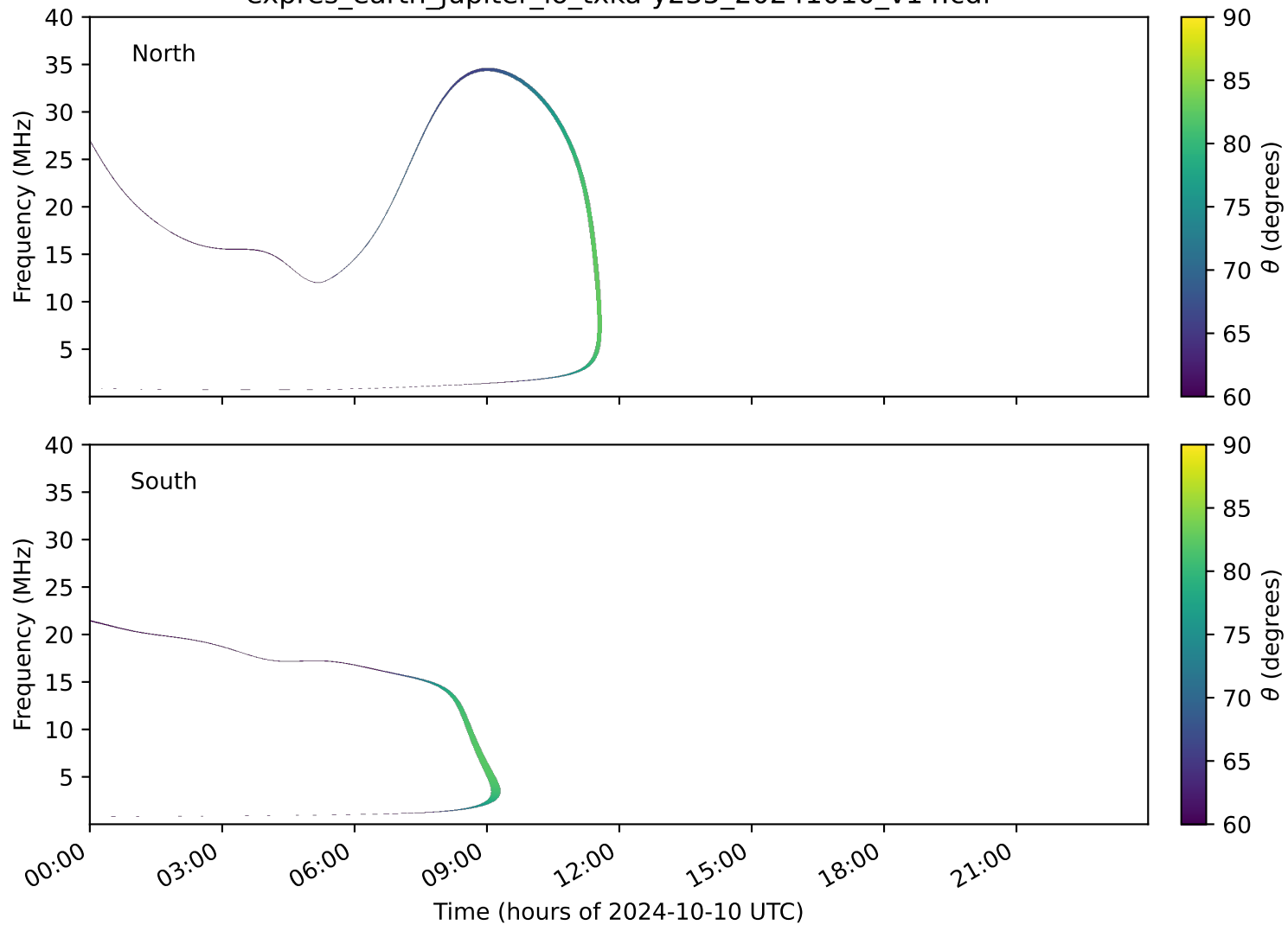
expres_earth_jupiter_io_txka-y235_20241010_v14.cdf
