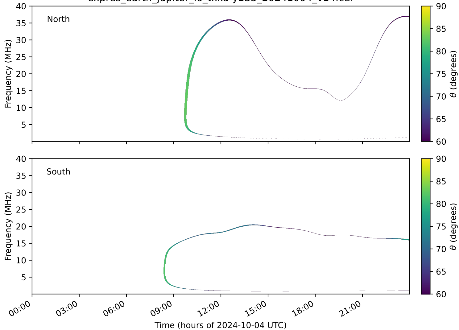
expres_earth_jupiter_io_txka-y235_20241004_v14.cdf
