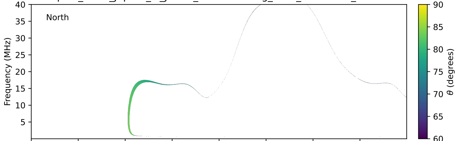
expres_earth_jupiter_io_jrm33_lossc-wid1deg_3kev_20241020_v11.cdf
