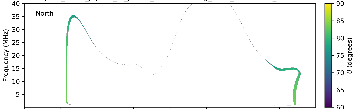
expres_earth_jupiter_io_jrm33_lossc-wid1deg_3kev_20241006_v11.cdf
