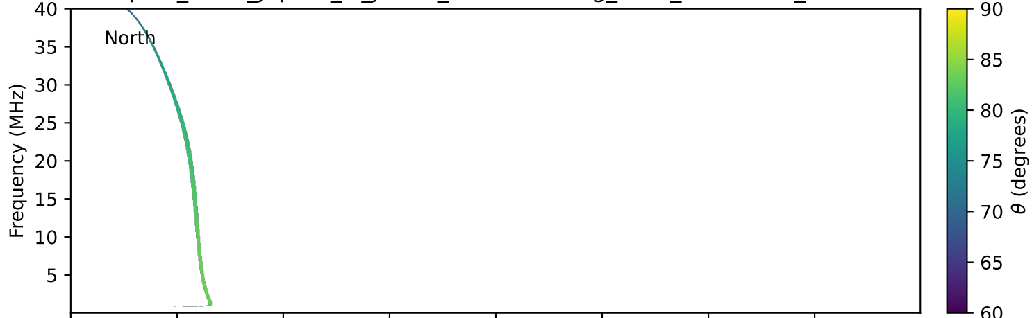
expres_earth_jupiter_io_jrm33_lossc-wid1deg_3kev_20241005_v11.cdf
