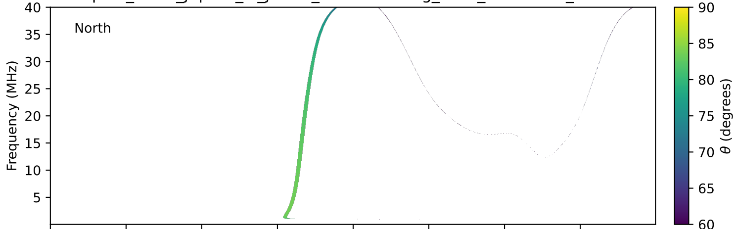
expres_earth_jupiter_io_jrm33_lossc-wid1deg_3kev_20241004_v11.cdf
