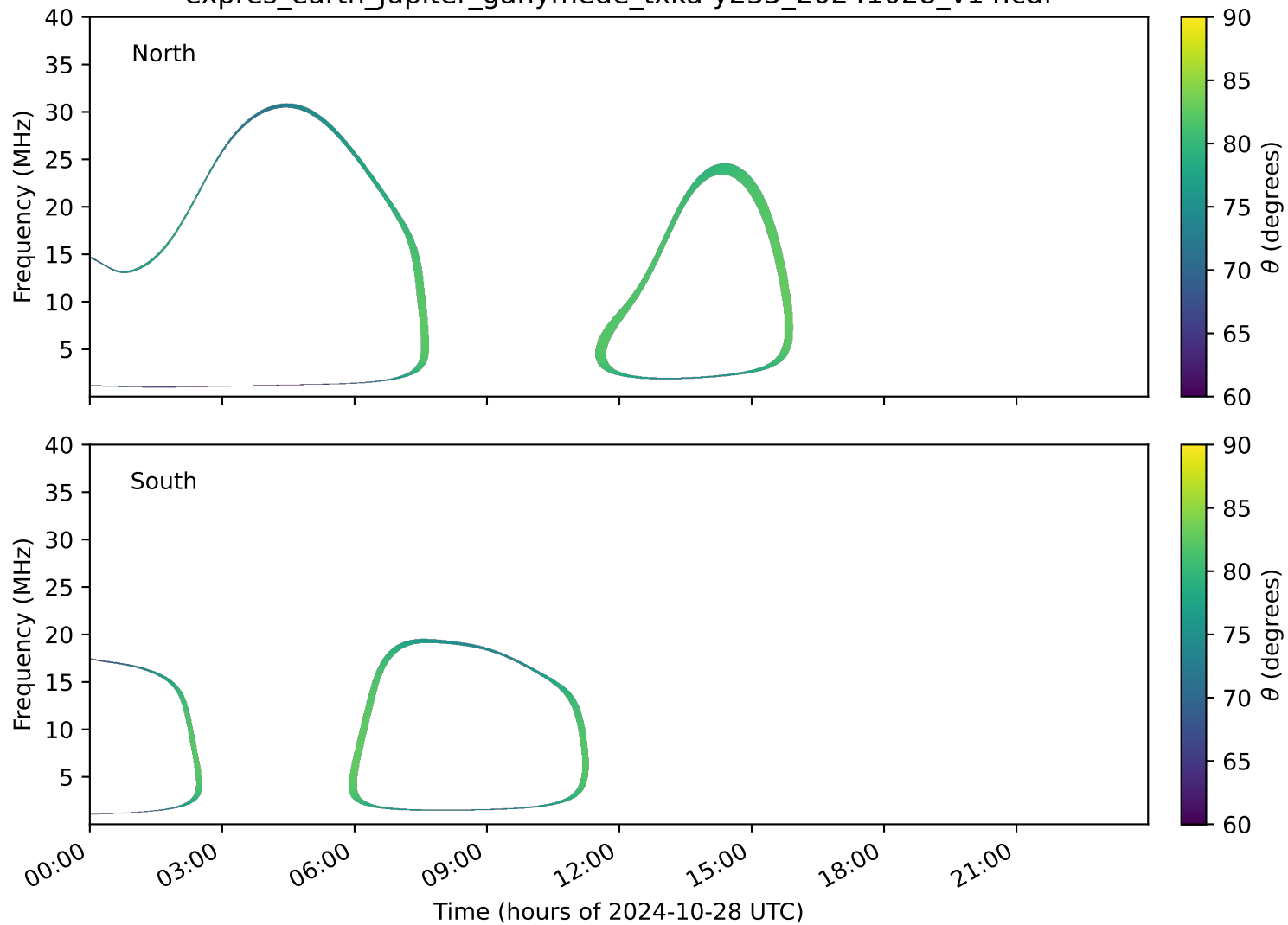
expres_earth_jupiter_ganymede_txka-y235_20241028_v14.cdf
