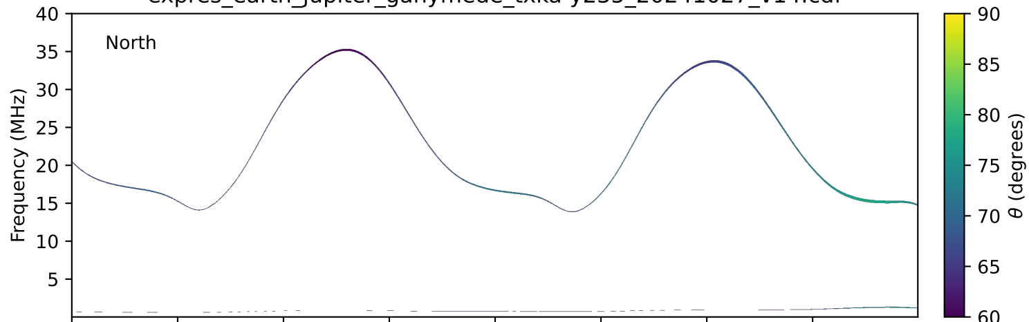
expres_earth_jupiter_ganymede_txka-y235_20241027_v14.cdf
