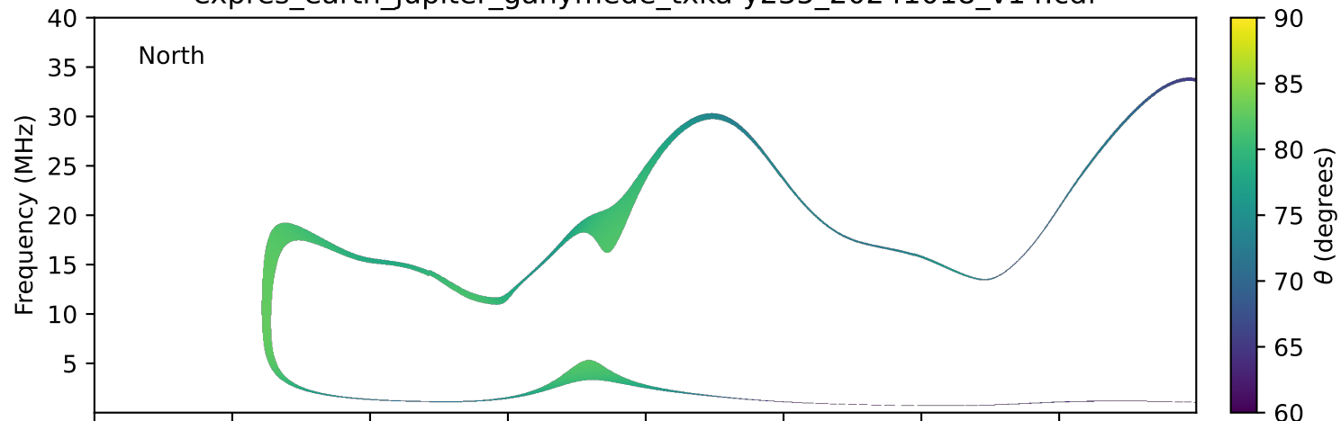
expres_earth_jupiter_ganymede_txka-y235_20241018_v14.cdf
