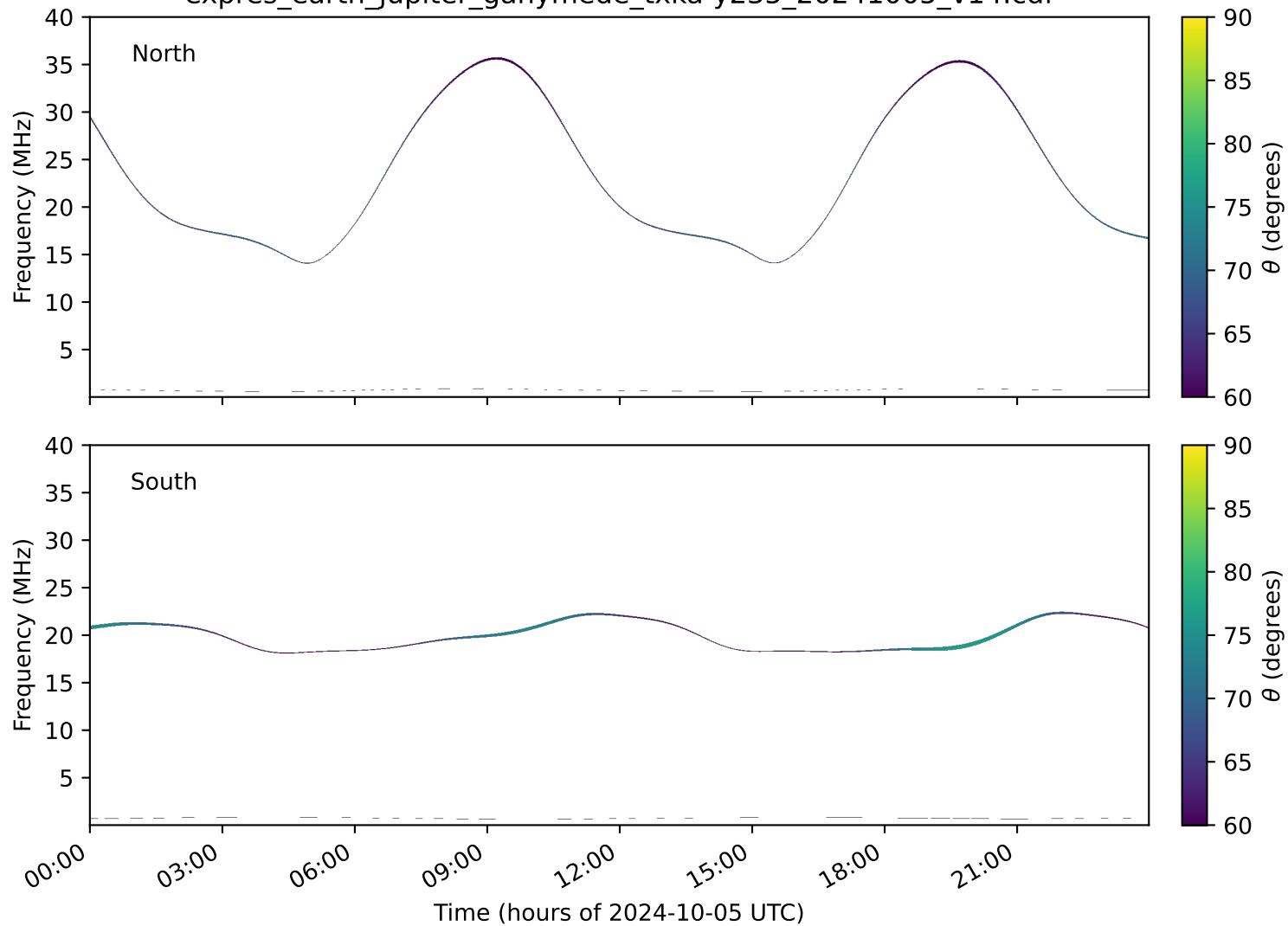
expres_earth_jupiter_ganymede_txka-y235_20241005_v14.cdf
