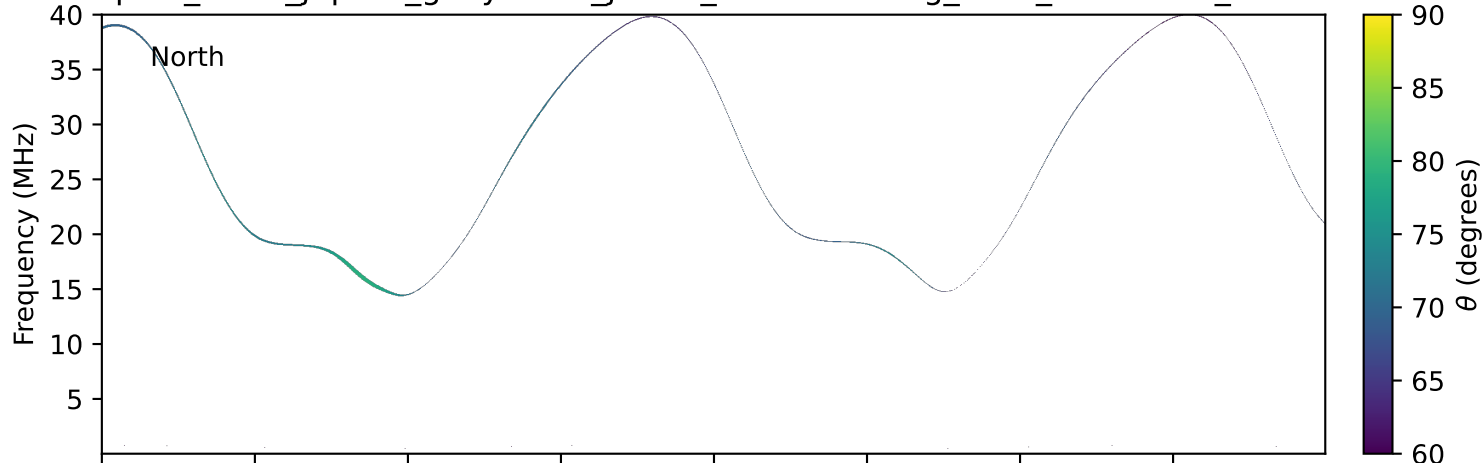
expres_earth_jupiter_ganymede_jrm33_lossc-wid1deg_3kev_20241026_v11.cdf
